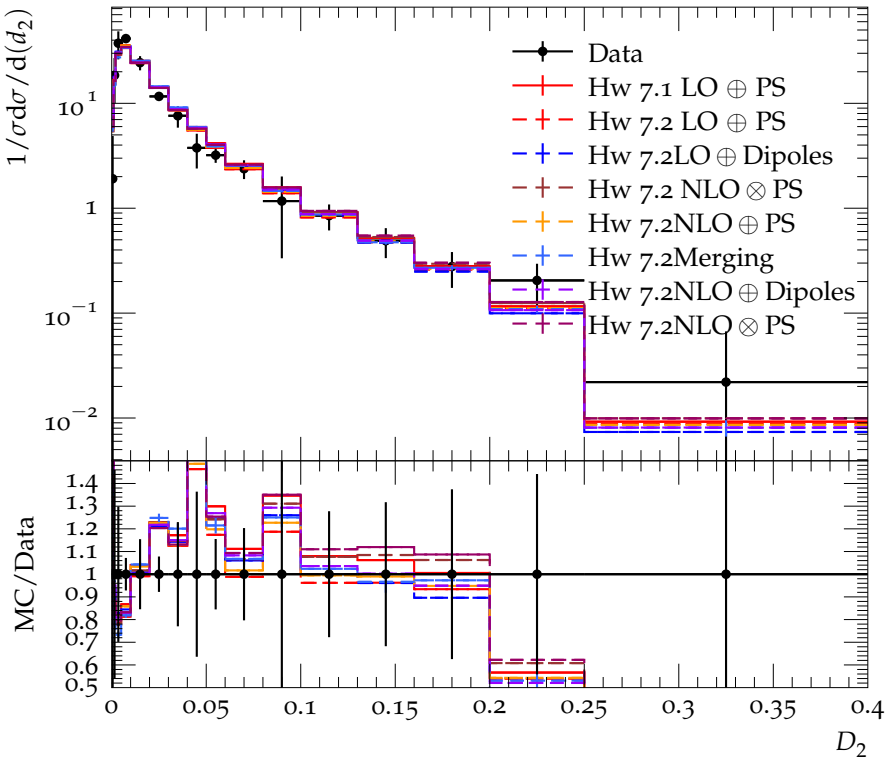
Differential 2-Jet rate (Durham), \sqrt{s} = 22 GeV
