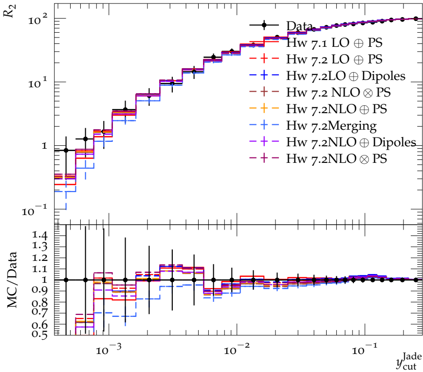
Integrated 2-jet rate with Jade algorithm (133 GeV)
