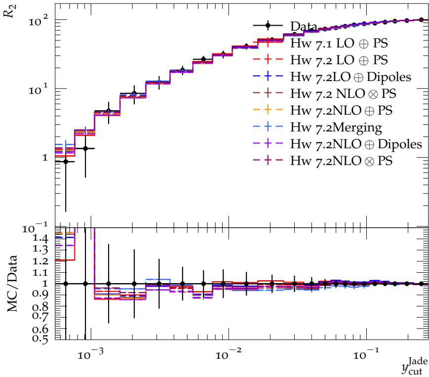
Integrated 2-jet rate with Jade algorithm (161 GeV)
