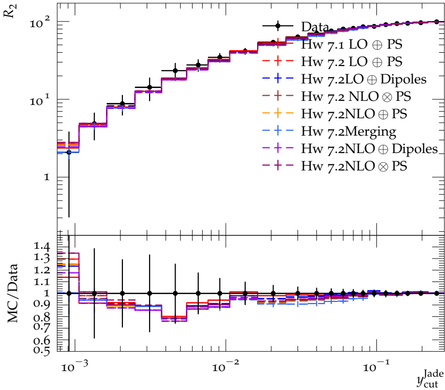
Integrated 2-jet rate with Jade algorithm (172 GeV)
