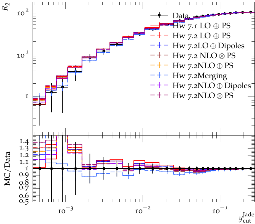
Integrated 2-jet rate with Jade algorithm (183 GeV)
