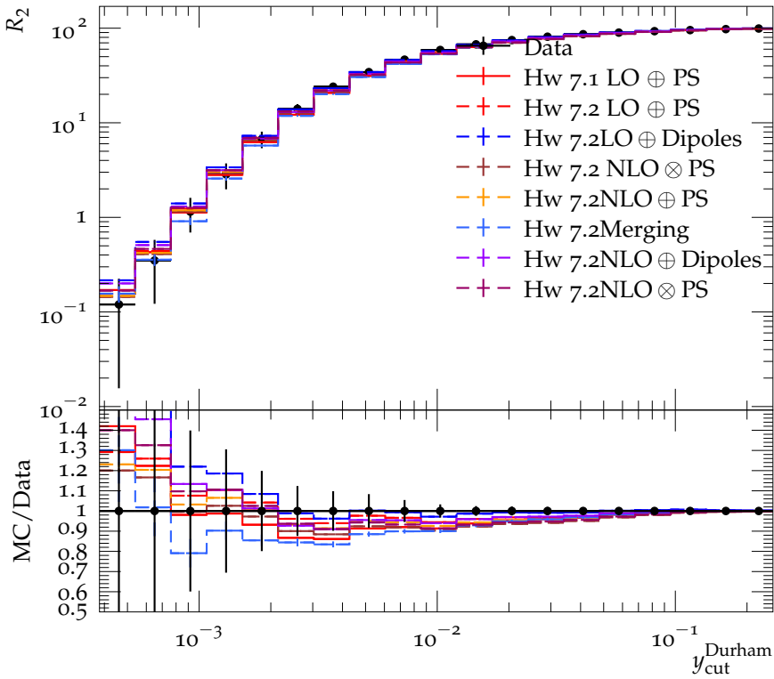
Integrated 2-jet rate with Durham algorithm (44 GeV)
