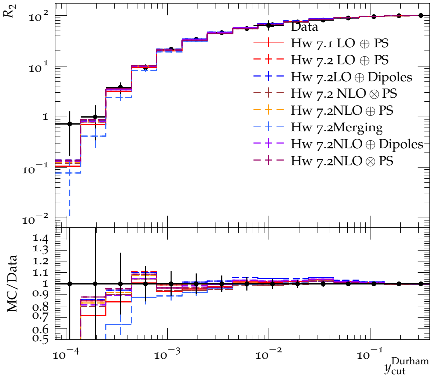
Integrated 2-jet rate with Durham algorithm (133 GeV)
