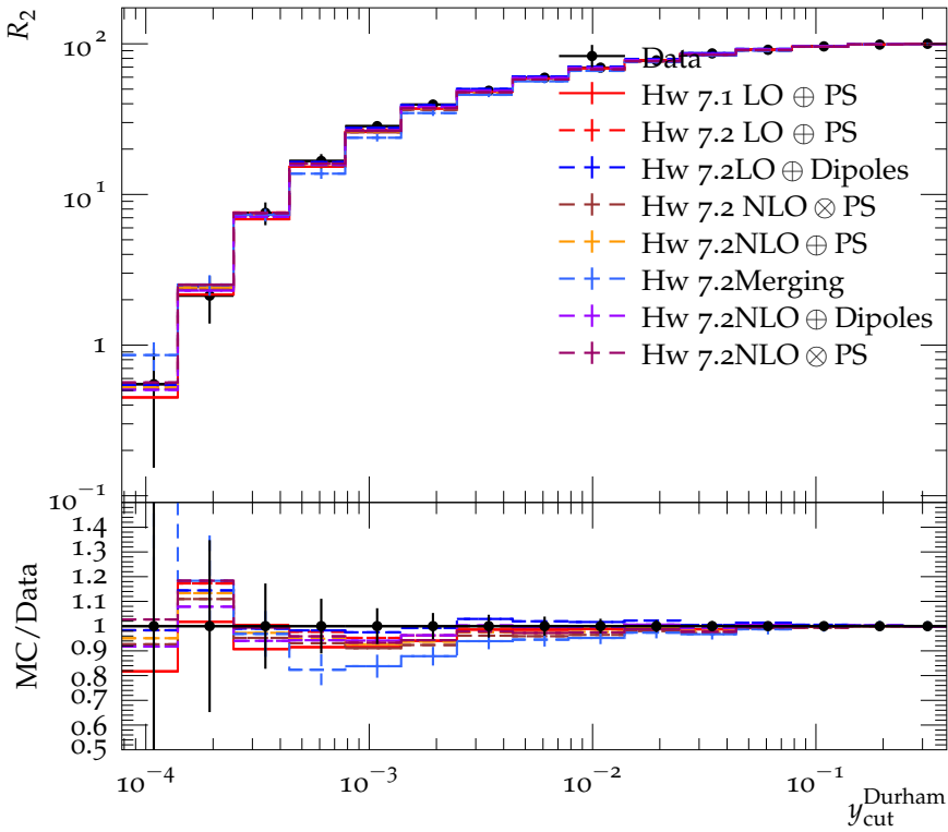
Integrated 2-jet rate with Durham algorithm (183 GeV)
