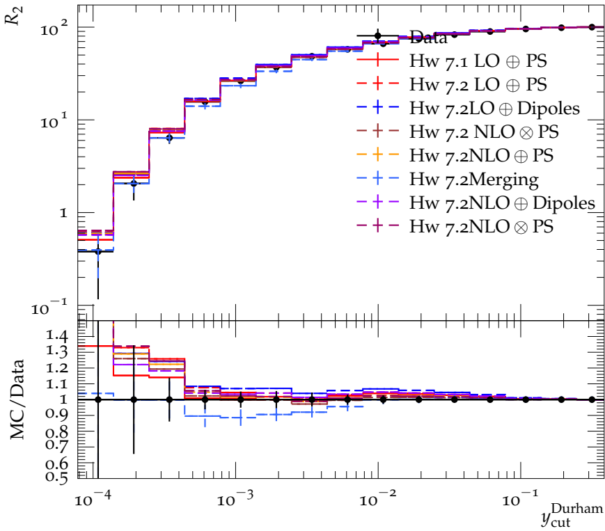
Integrated 2-jet rate with Durham algorithm (189 GeV)
