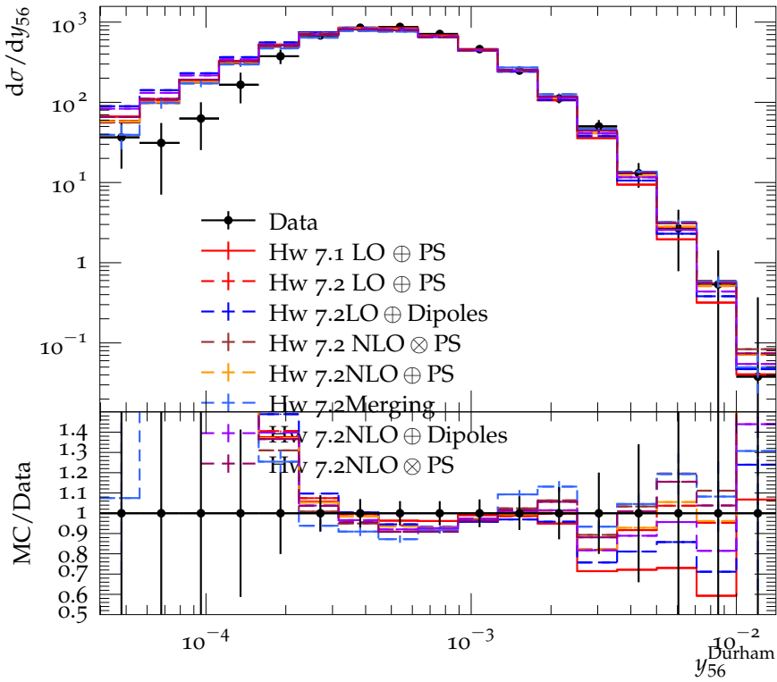
Differential 5-jet rate with Durham algorithm (44 GeV)
