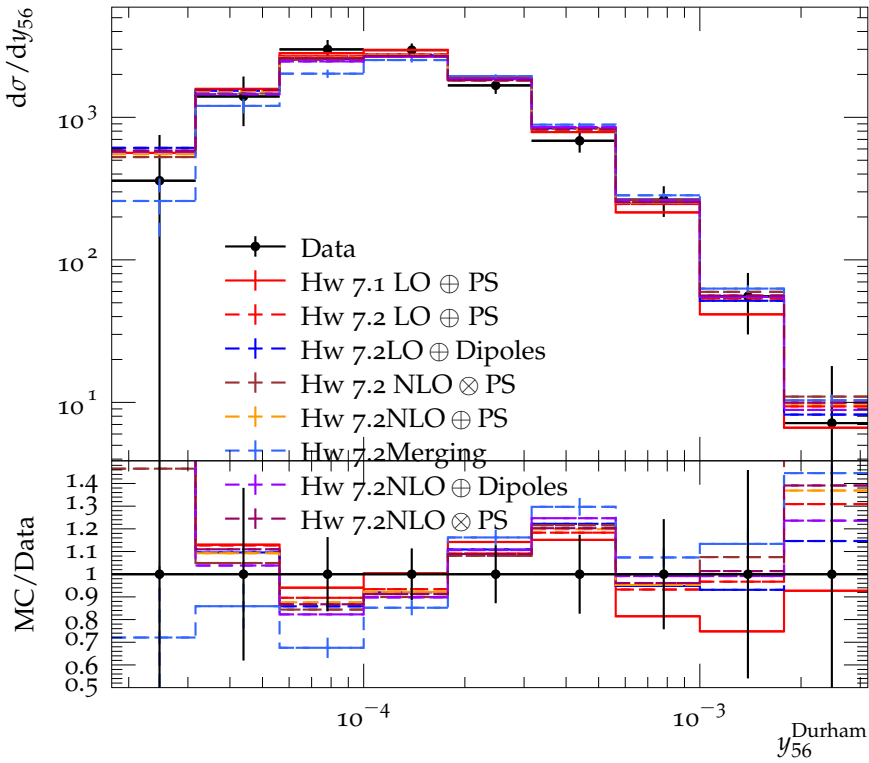
Differential 5-jet rate with Durham algorithm (133 GeV)
