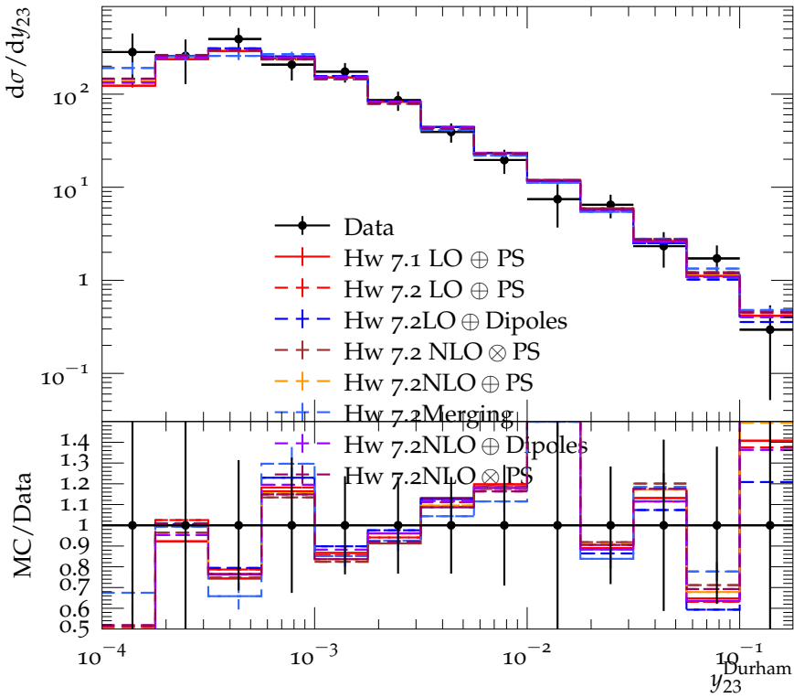
Differential 2-jet rate with Durham algorithm (161 GeV)
