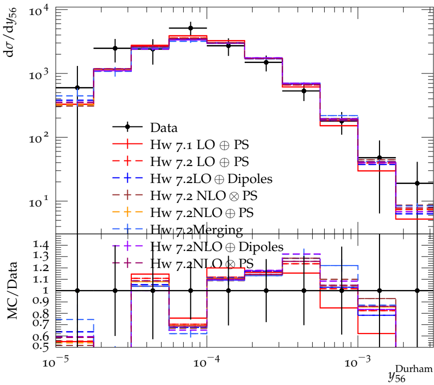
Differential 5-jet rate with Durham algorithm (161 GeV)
