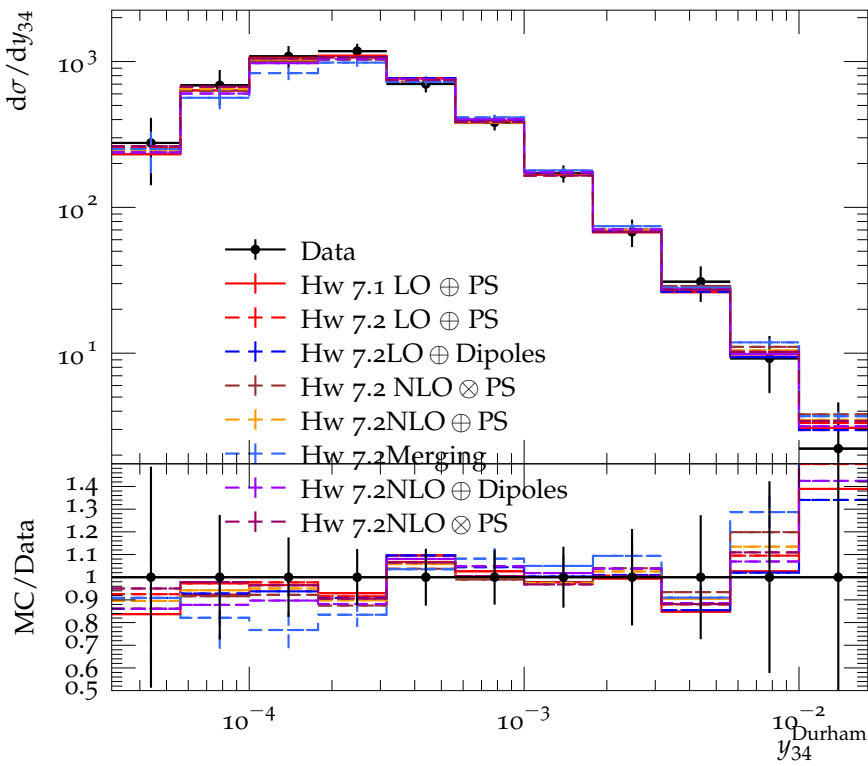
Differential 3-jet rate with Durham algorithm (183 GeV)
