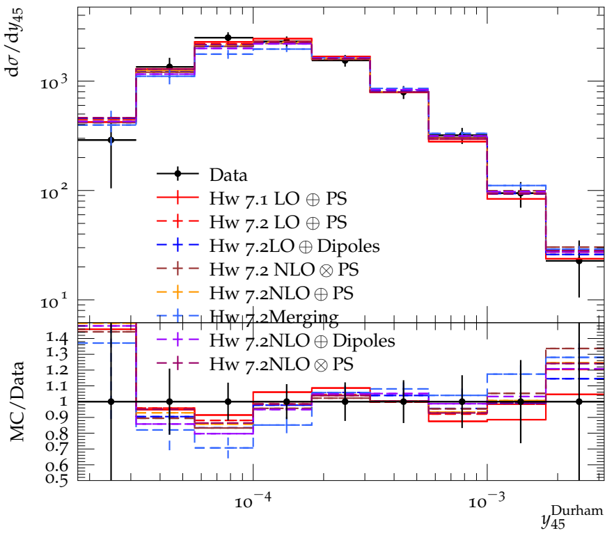
Differential 4-jet rate with Durham algorithm (183 GeV)
