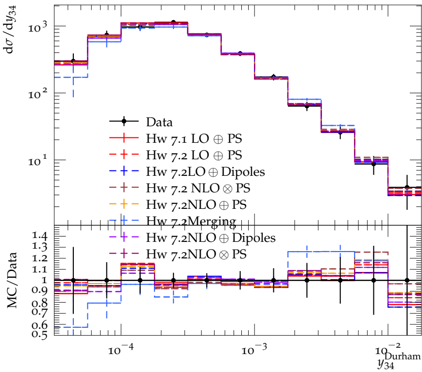
Differential 3-jet rate with Durham algorithm (189 GeV)
