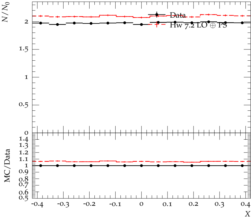
Dalitz plot slice for -0.8 < Y < -0.7
