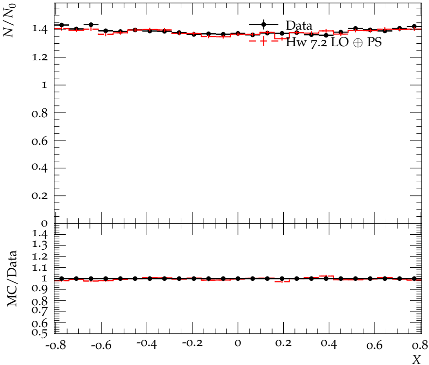
Dalitz plot slice for -0.3 < Y < -0.2
