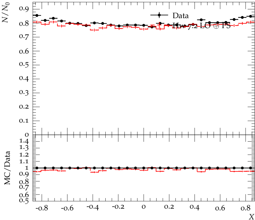
Dalitz plot slice for 0.2 < Y < 0.3
