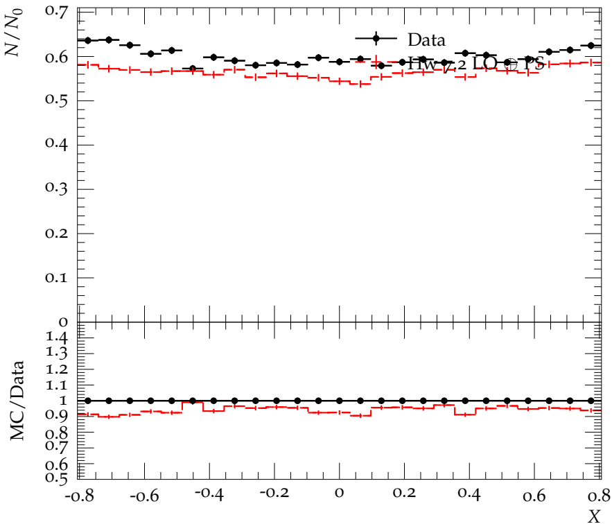
Dalitz plot slice for 0.4 < Y < 0.5
