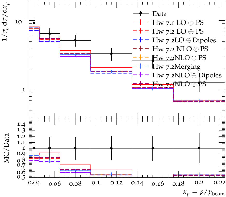
The x_p spectrum for inclusive \eta production at the Z^0 resonance
