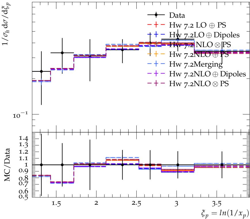
The \xi_p spectrum for \omega production at the Z^0 resonance
