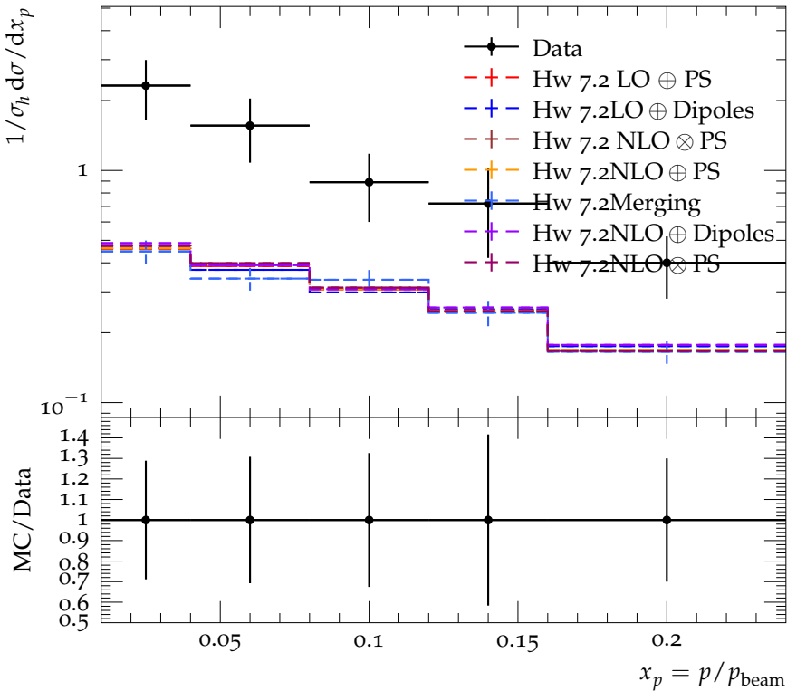
The x_p spectrum for \eta' (using \eta' \rightarrow \rho^0 \gamma ) at the Z^0 resonance
