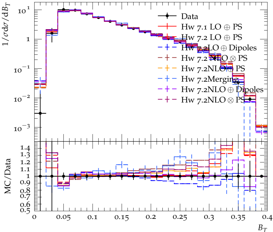
Total jet broadening, udsc events, at E_{\text{CMS}} = 91.2 GeV
