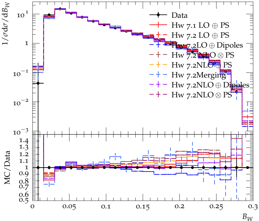
Wide jet broadening, udsc events, at E_{\text{CMS}} = 91.2 GeV
