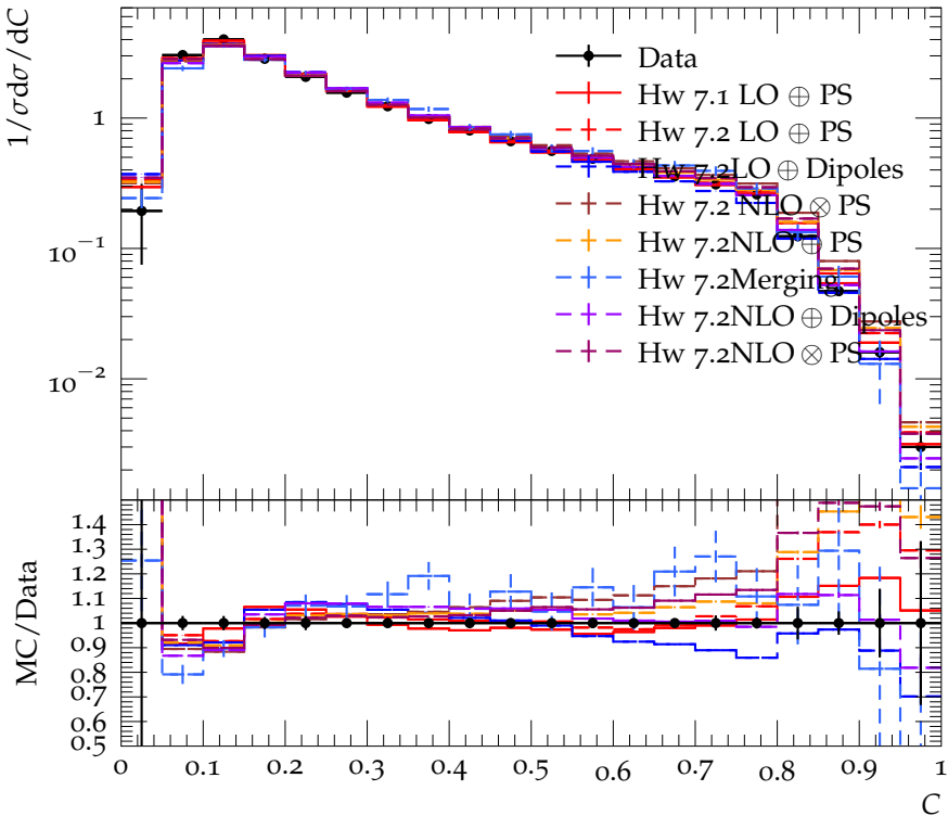
C-parameter, udsc events, at E_{\text{CMS}} = 91.2 GeV
