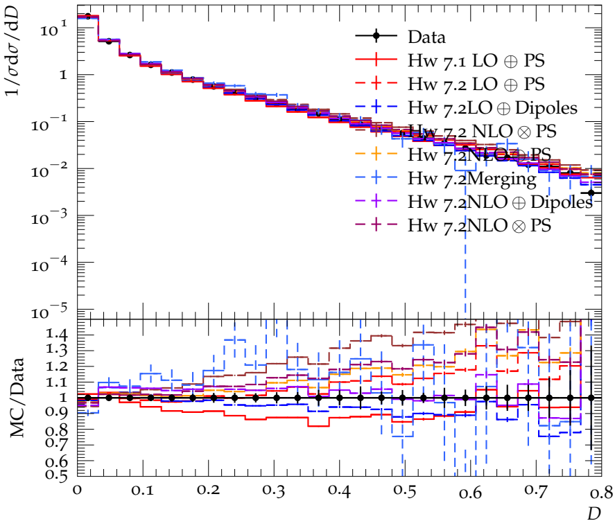
D-parameter, udsc events, at E_{\text{CMS}} = 91.2 GeV
