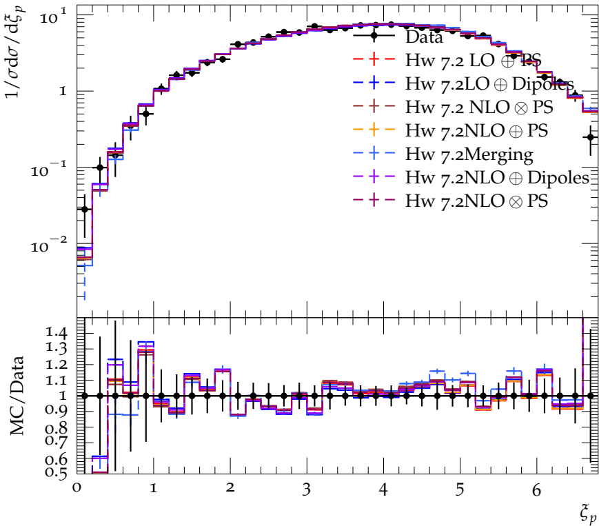
Log of scaled momentum distribution at E_{\text{CMS}} = 161.3 GeV
