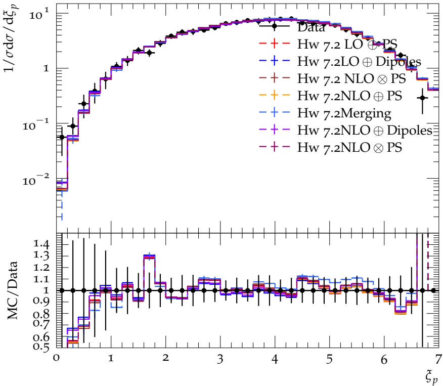
Log of scaled momentum distribution at E_{\text{CMS}} = 172.3 GeV
