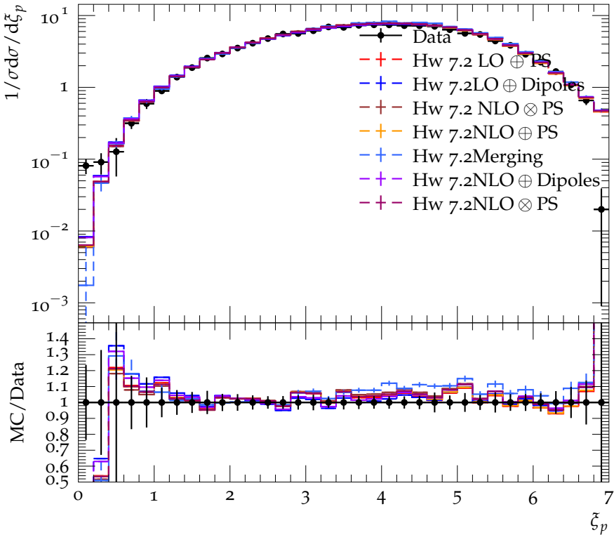
Log of scaled momentum distribution at E_{\text{CMS}} = 182.8 GeV
