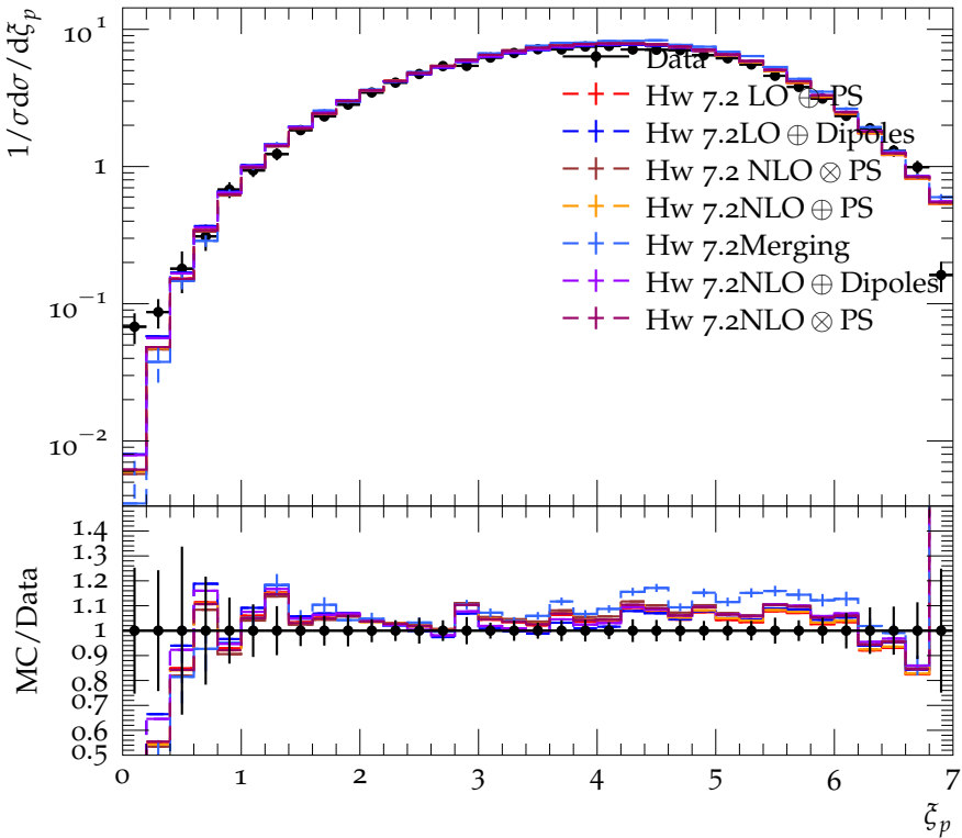
Log of scaled momentum distribution at E_{\text{CMS}} = 194.4 GeV
