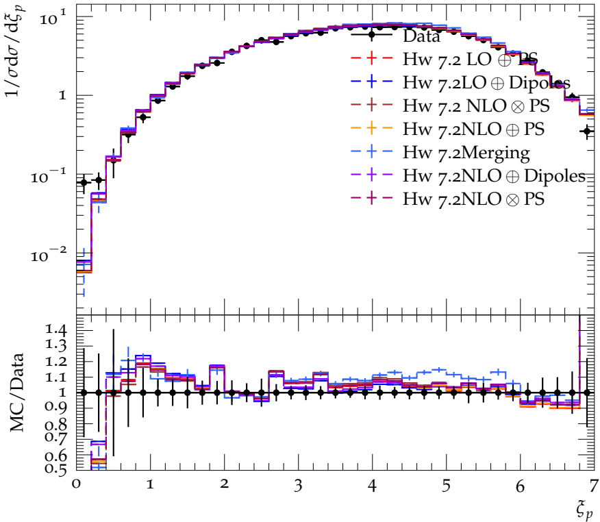
Log of scaled momentum distribution at E_{\text{CMS}} = 200.2 GeV
