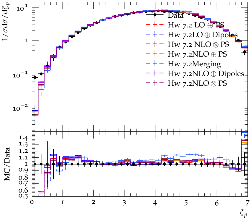
Log of scaled momentum distribution at E_{\text{CMS}} = 206.2 GeV
