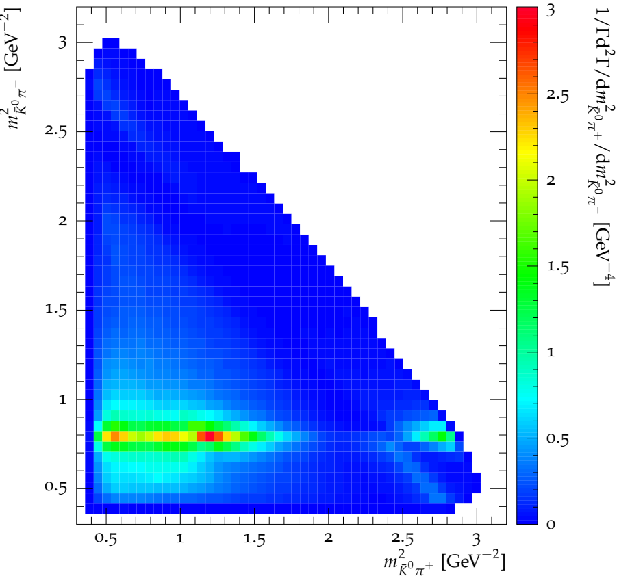
Dalitz plot for D^0 \rightarrow \bar{K}^0 \pi^+ \pi^-
