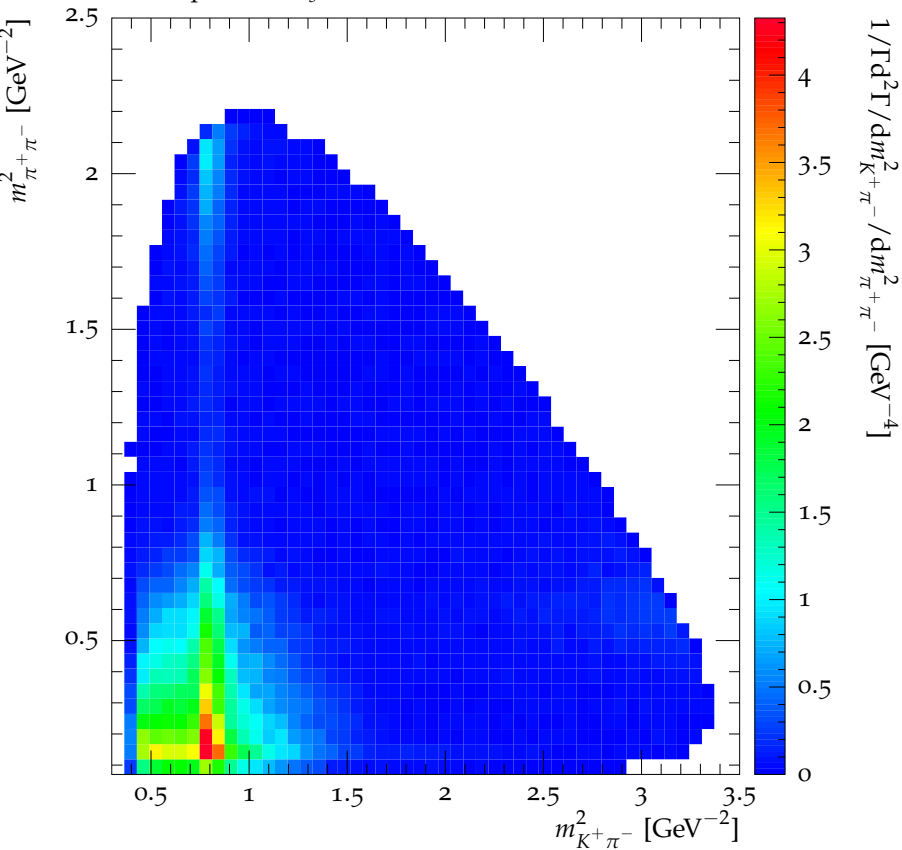
Dalitz plot for D_s^+ \rightarrow K^+ \pi^- \pi^+
