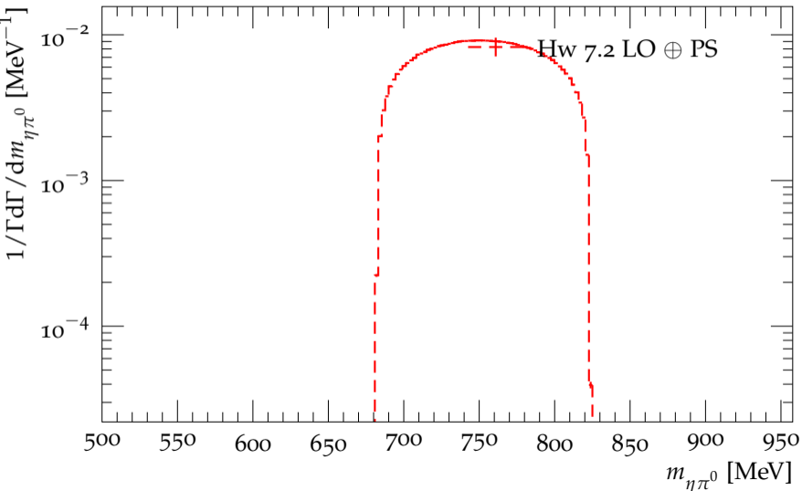
Distribution of the \eta\pi^0 mass in the decay \eta' \rightarrow \eta\pi^0\pi^0
