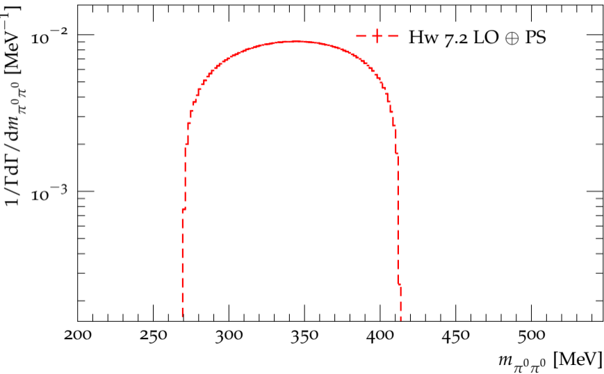
Distribution of the \pi\pi^0 mass in the decay \eta \rightarrow \pi^0\pi^0\pi^0
