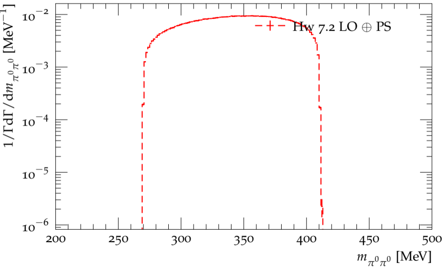
Distribution of the \pi^0\pi^0 mass in the decay \eta' \rightarrow \eta\pi^0\pi^0
