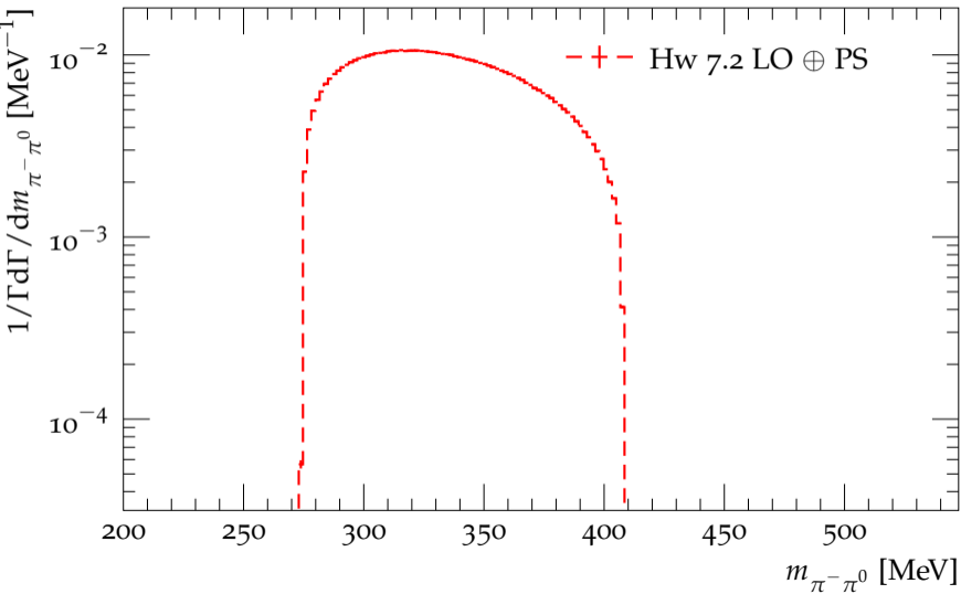
Distribution of the \pi^- \pi^0 mass in the decay \eta \rightarrow \pi^+ \pi^- \pi^0
