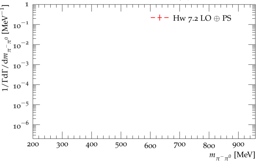
Distribution of the \pi^- \pi^0 mass in the decay \eta' \rightarrow \pi^+ \pi^- \pi^0
