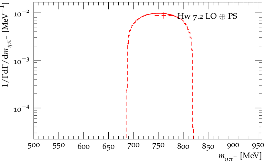
Distribution of the \eta\pi^- mass in the decay \eta' \rightarrow \eta\pi^+\pi^-
