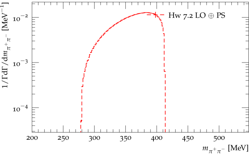
Distribution of the \pi^+\pi^- mass in the decay \eta \rightarrow \pi^+\pi^-\pi^0
