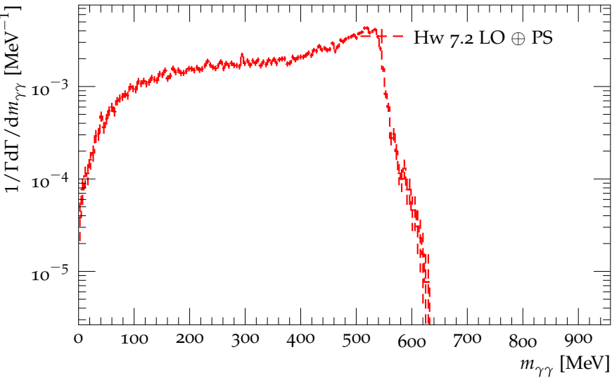
Distribution of the \gamma\gamma mass in the decay \eta' \rightarrow \gamma\gamma\pi^0
