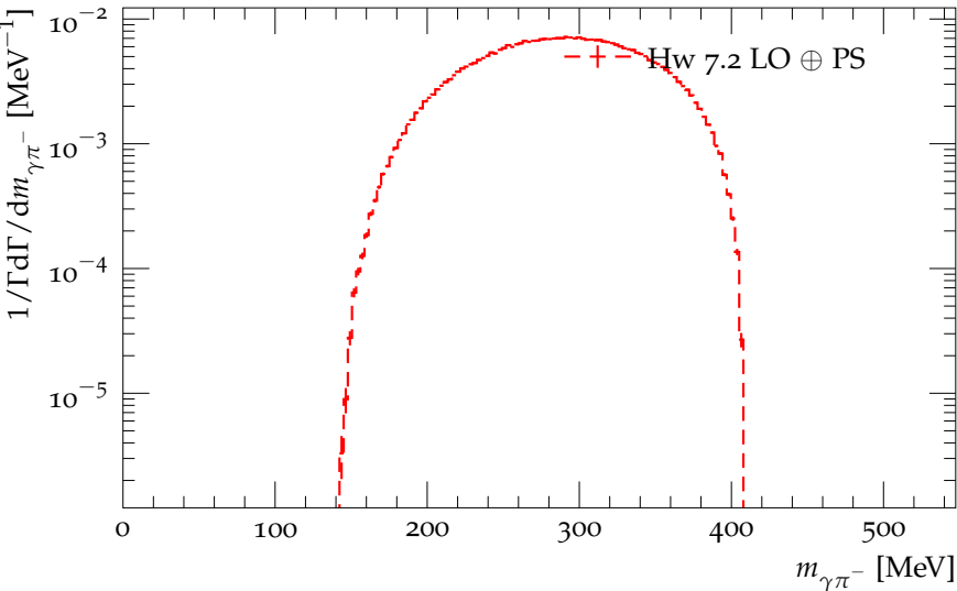
Distribution of the \gamma\pi^- mass in the decay \eta \rightarrow \gamma\pi^+\pi^-
