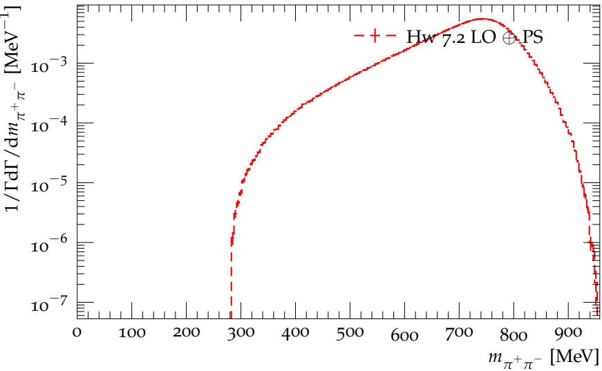
Distribution of the \pi^+\pi^- mass in the decay \eta' \rightarrow \gamma\pi^+\pi^-
