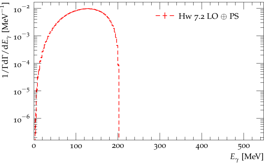
Distribution of the photon energy in the decay \eta \rightarrow \gamma\pi^+\pi^-
