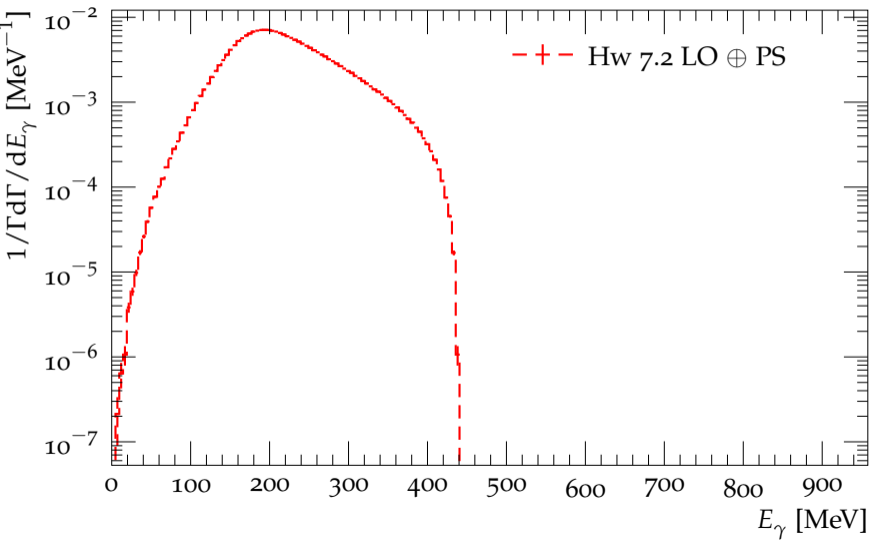
Distribution of the photon energy in the decay \eta' \rightarrow \gamma\pi^+\pi^-
