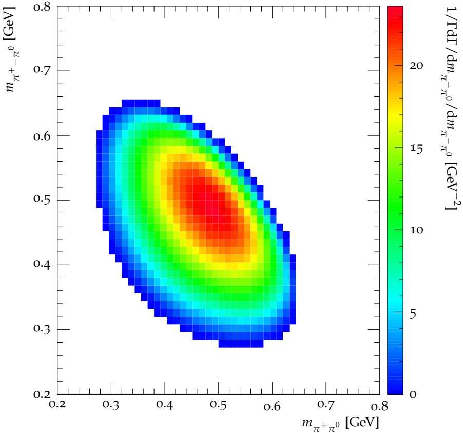
Dalitz plot for \omega \rightarrow \pi^0 \pi^+ \pi^- decays
