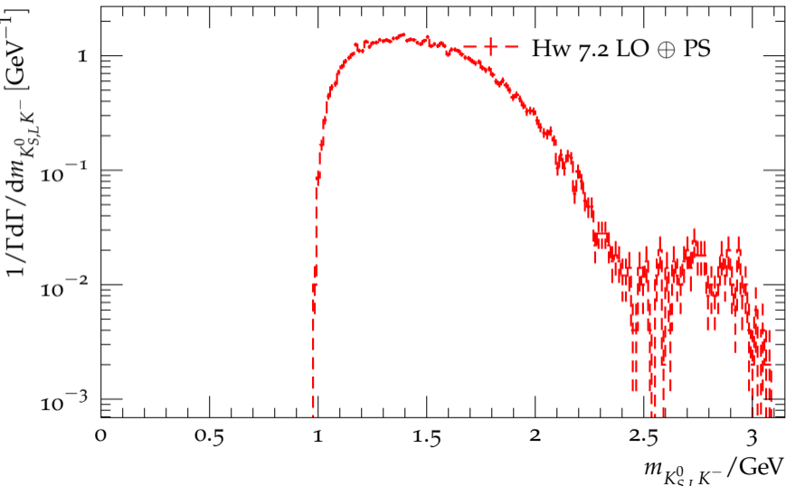
Mass distribution of the hadrons for \tau^- \rightarrow K_{S,L}^0 K^- \nu_\tau
