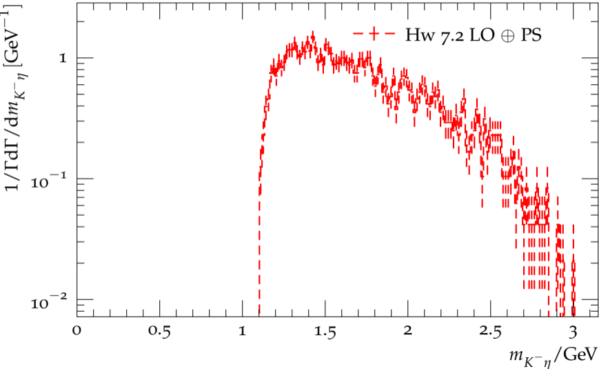
Mass distribution of the hadrons for \tau^- \rightarrow K^- \eta \nu_\tau
